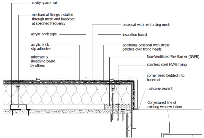
Diagram 10 - Typical window/door head detail
