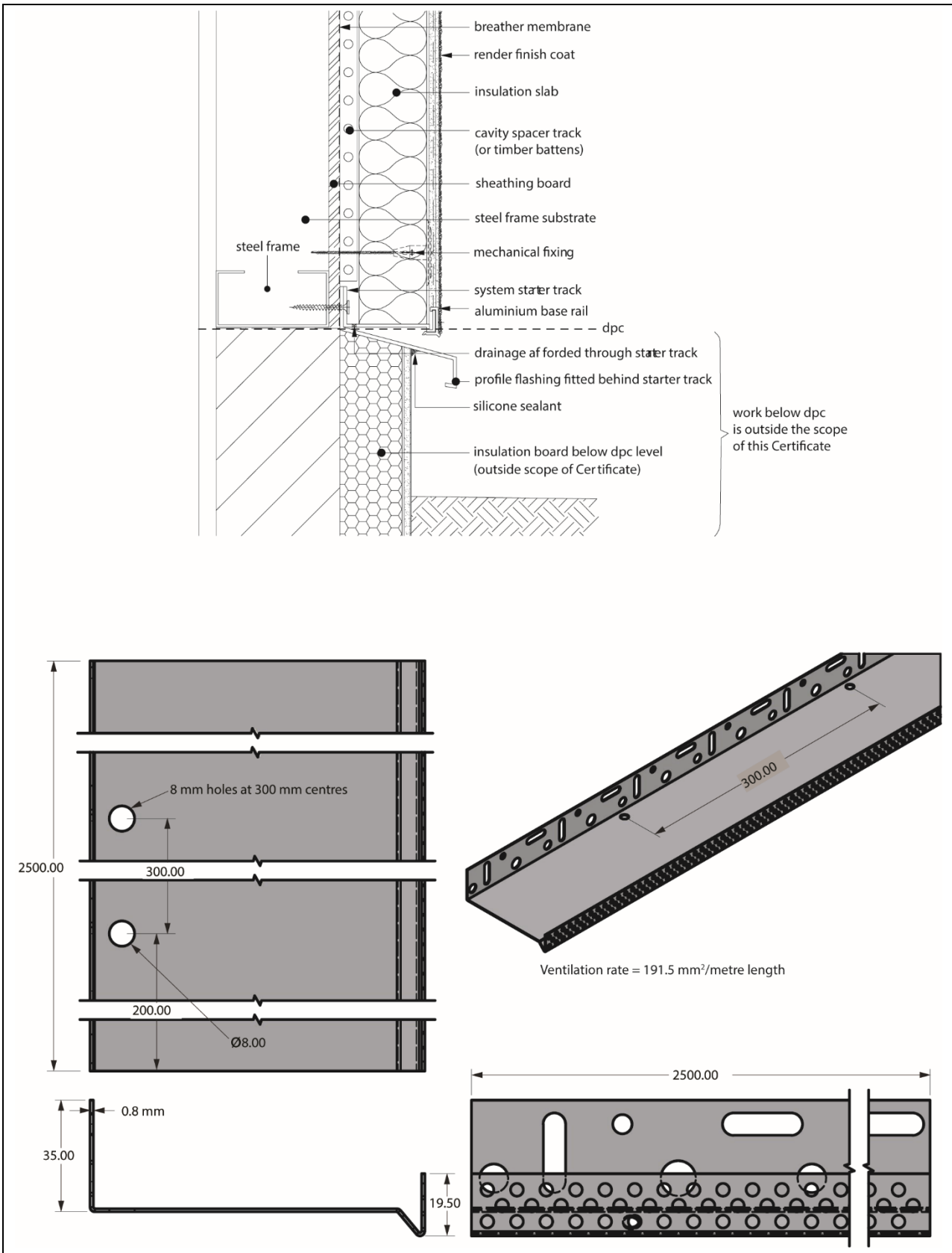
Figure 3 Typical section of base rail
