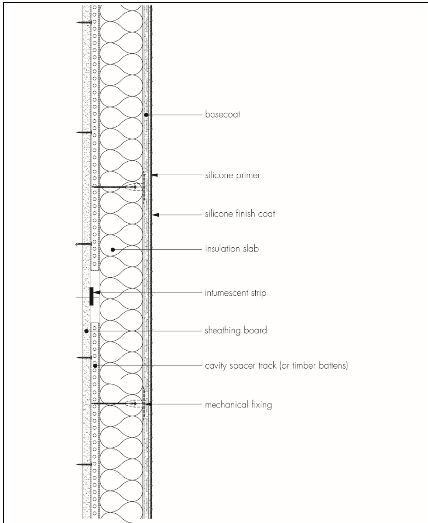
Figure 3 Fire barriers
