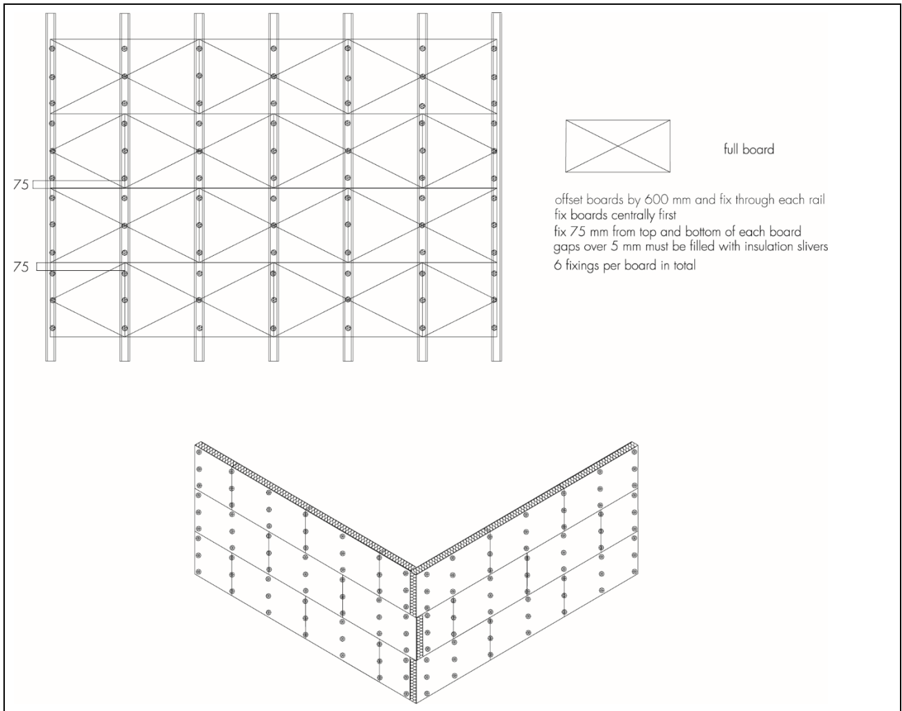
Figure 4 Arrangement of insulation slabs and typical fixing pattern
