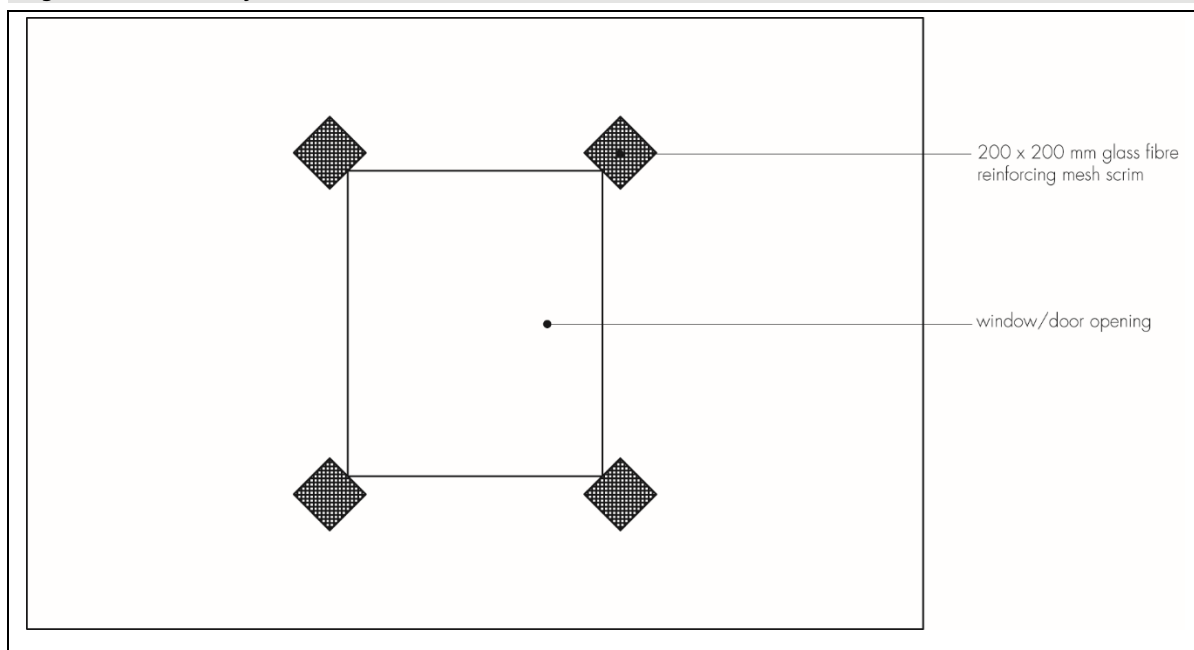
Figure 8 Corner reinforcement
