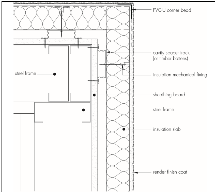
Figure 5 Typical corner detail
