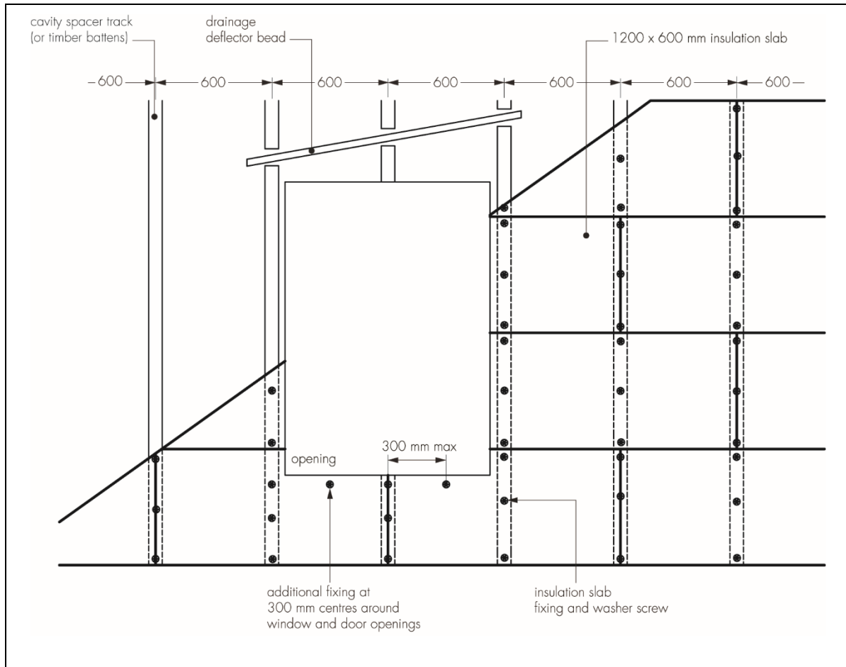
Figure 6 Typical opening details showing deflection channel
