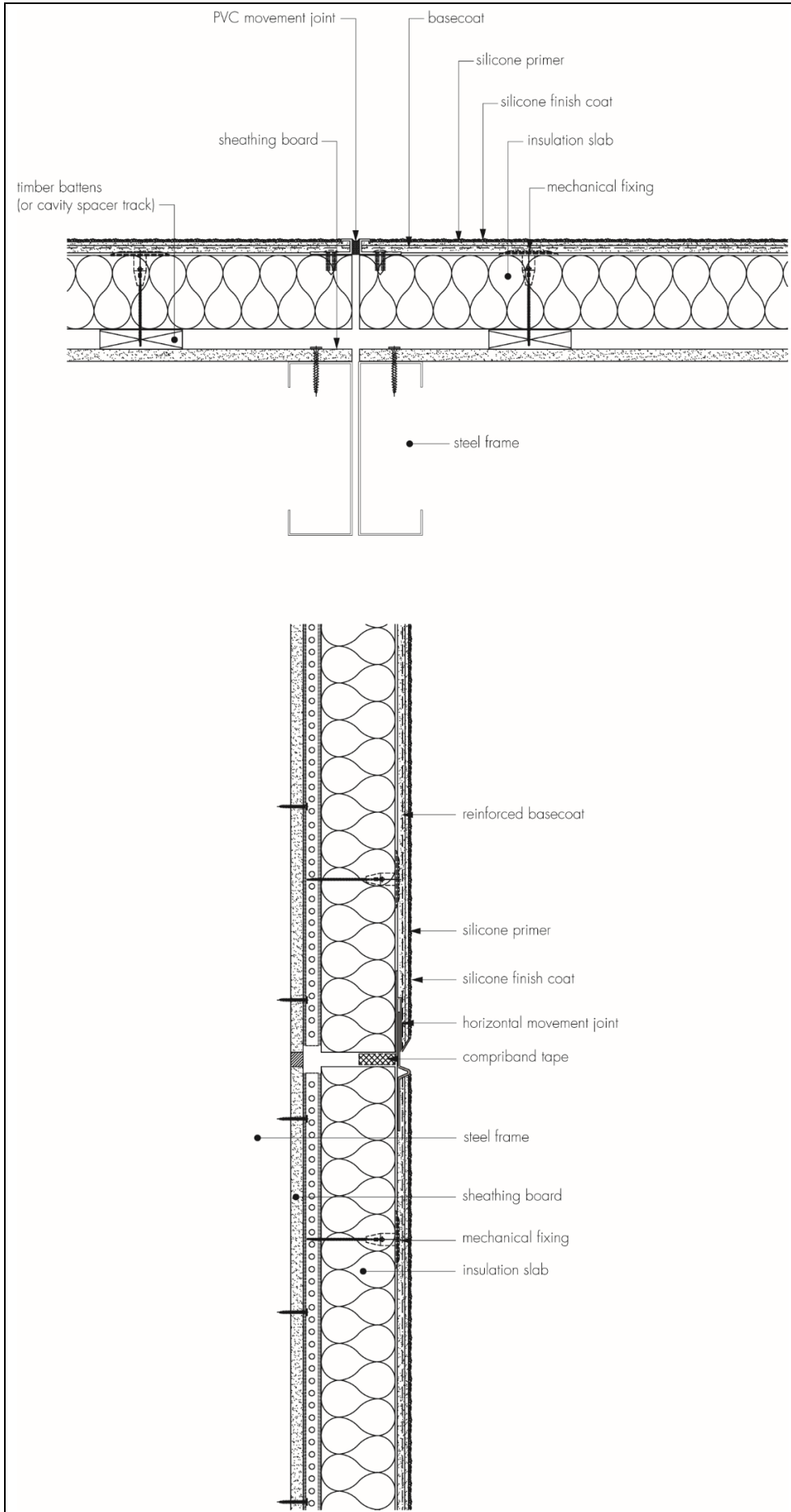
Figure 7 Vertical and horizontal movement joint details
