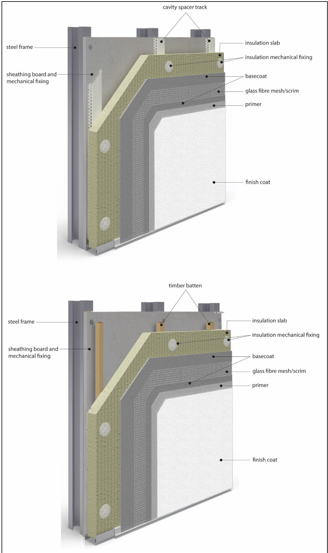
Figure 1 Epsitec Stone Wool External Wall Insulation System for Steel Framed Buildings through steel spacer rails (top-hat sections) or timber battens
