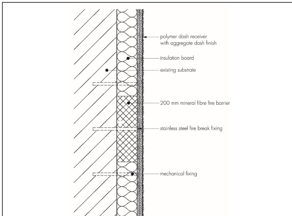
Figure 2 Fire barrier
