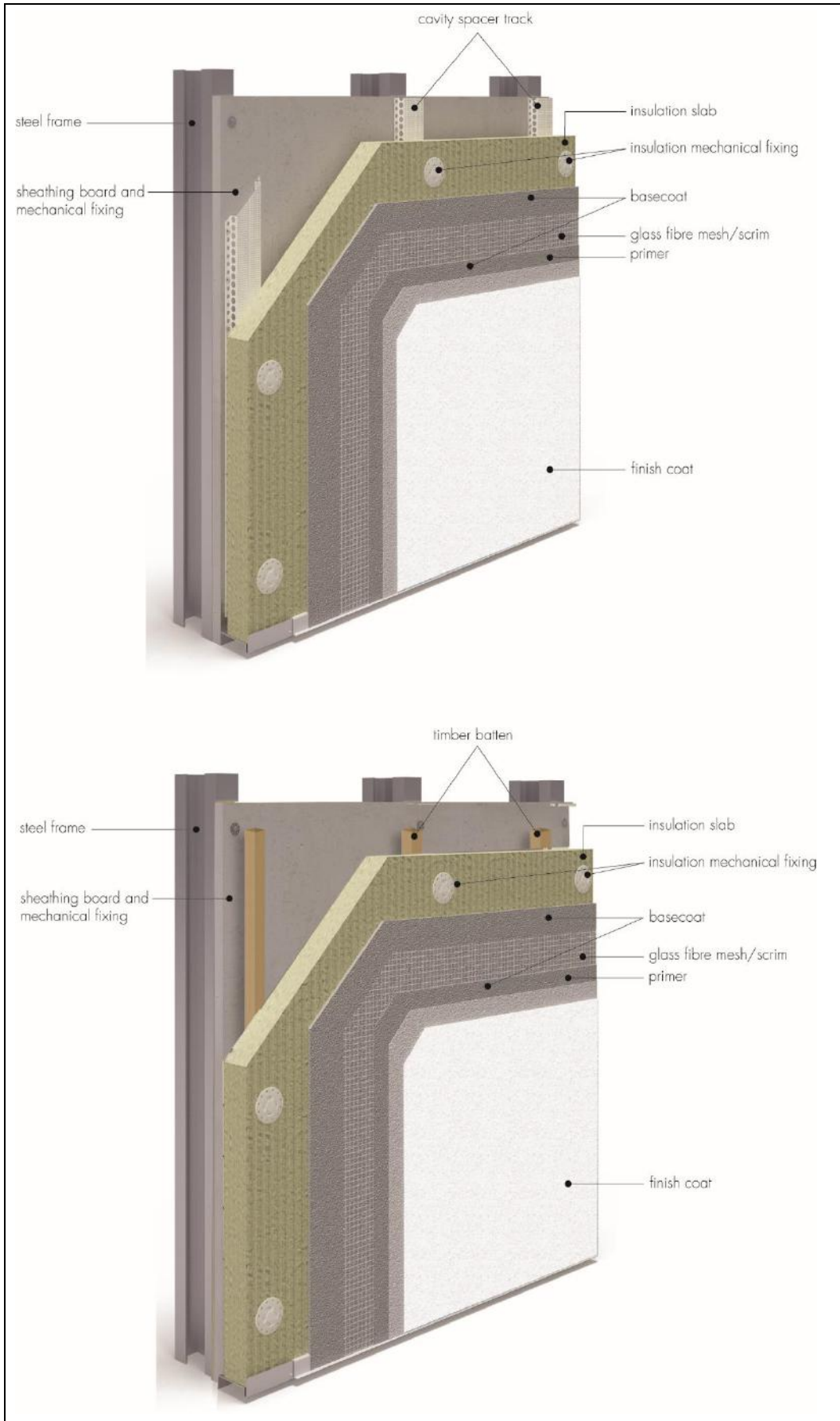
Figure 1 Epsitec Stone Wool External Wall Insulation System for Steel Framed Buildings through steel spacer rails (top-hat sections) or timber battens
