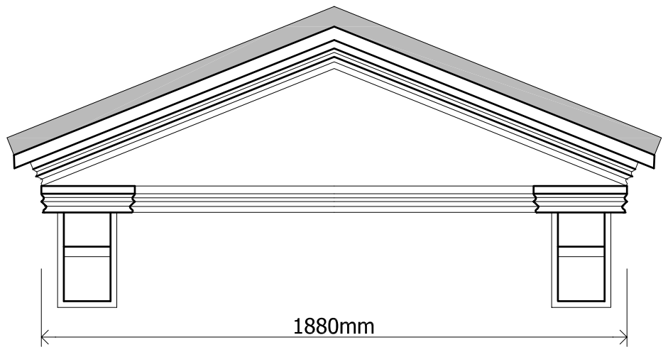
Front Elevation
